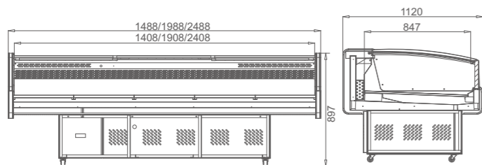
DLCD-1.5PF-B / DLCD-2.0PF-B / DLCD-2.5PF-B
