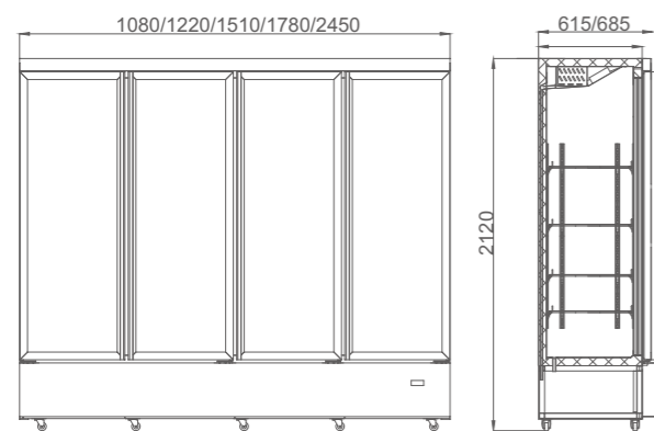
LG-882M2/WP / LG-1000M2/WP / LG-1200M3/WP / LG-1400M3/WP / LG-1800M4/WP
